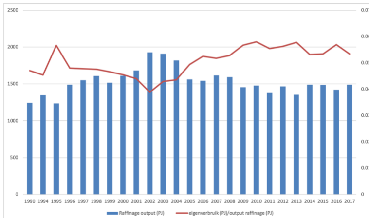
Figure 28: The refining total output (PJ) and the energy use in refining per unit of output (Source: VITO, 2019)
