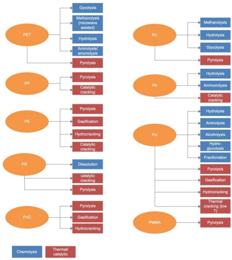
Figure 45: Options for chemical recycling for important polymers
